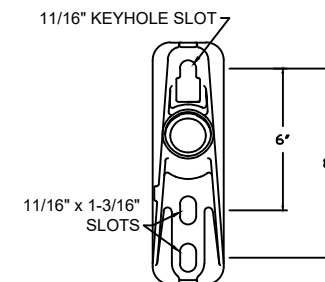
BASE VIEW
